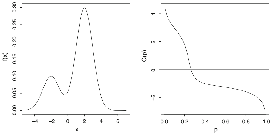
Fig. 1 Density of 0.25N(-2, 1) + 0.75N(2, 1) and the corresponding cross-over function G(p)
